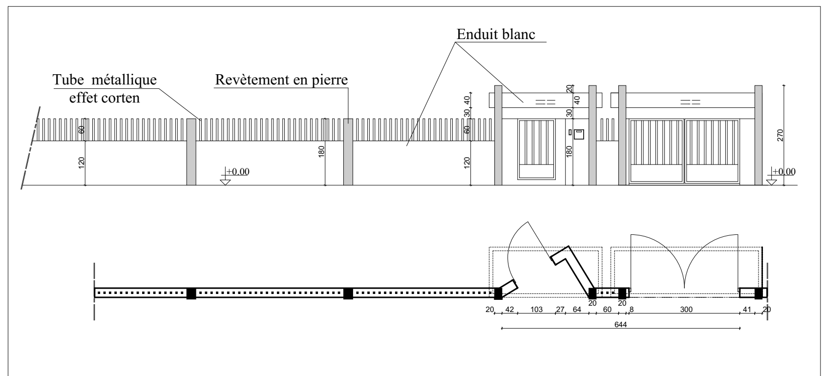
DETAIL MUR CLOTURE
