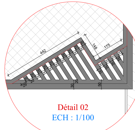
DETAIL MUR CLOTURE
